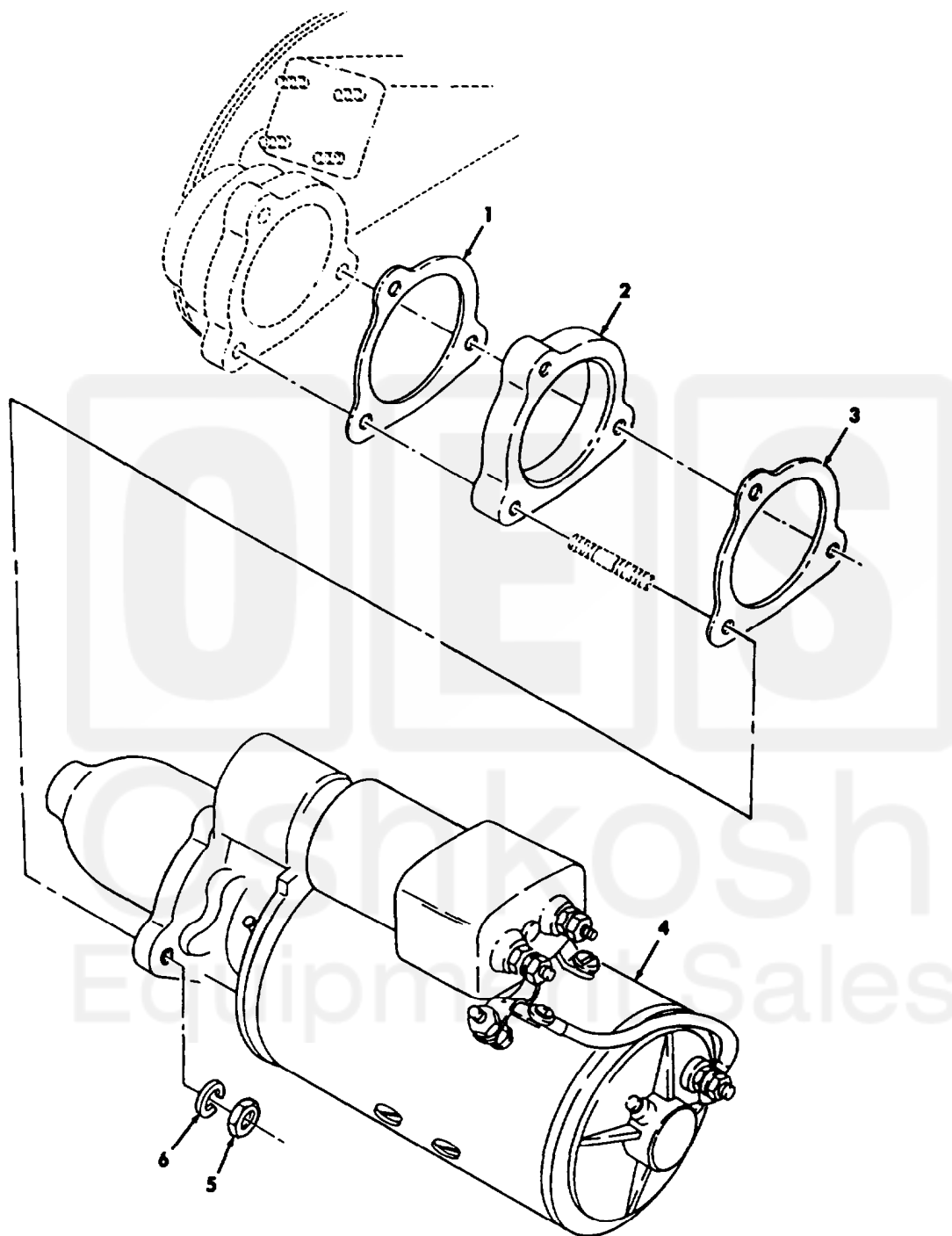
Figure 32. Starting Motor and Related Parts.
